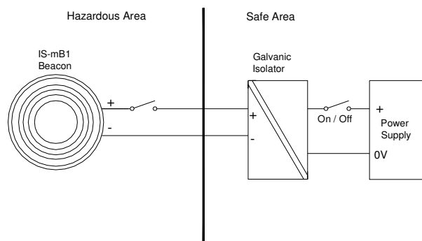
Fig 5 Basic circuit for use with a galvanic isolator.
